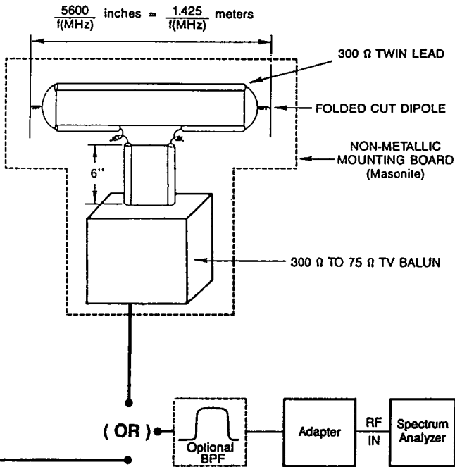
Figure 4-5. Equipment setup for field strength measurements.
