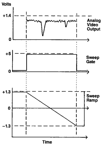
Figure 5-1. Sweep gate and ramp timing.
