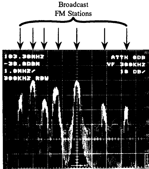
Figure 4-11. Portion of US broadcast FM band.
