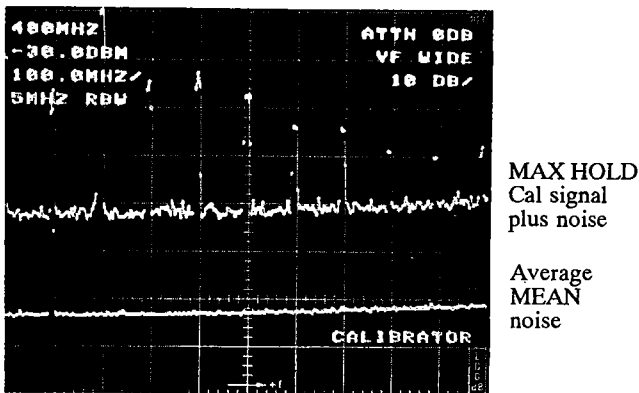
Figure 4-7. Average MEAN noise and MAX HOLD signal plus noise spectra.
