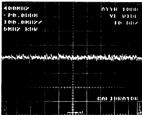
Figure 4-6. Average signal plus noise and average signal plus noise subtracted from the current sweep.
