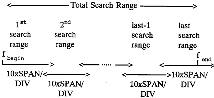
Figure 4-14. The SIGNAL SEARCH frequency range.
