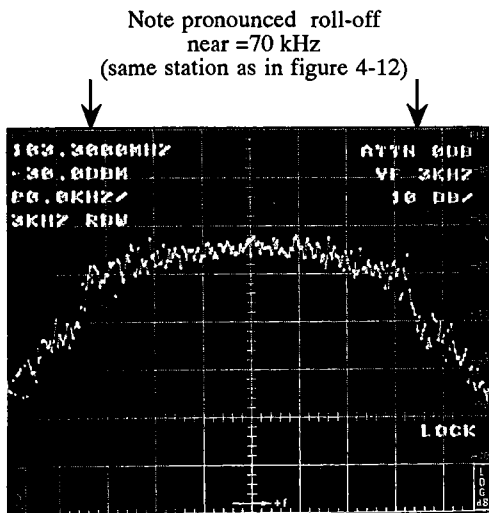
Figure 4-13. Frequency deviation by MAX HOLD technique.
