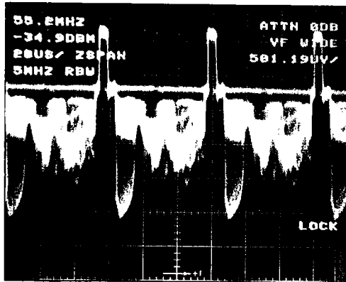
Figure 4-17. Video signal using continuous horizontal line triggering.
