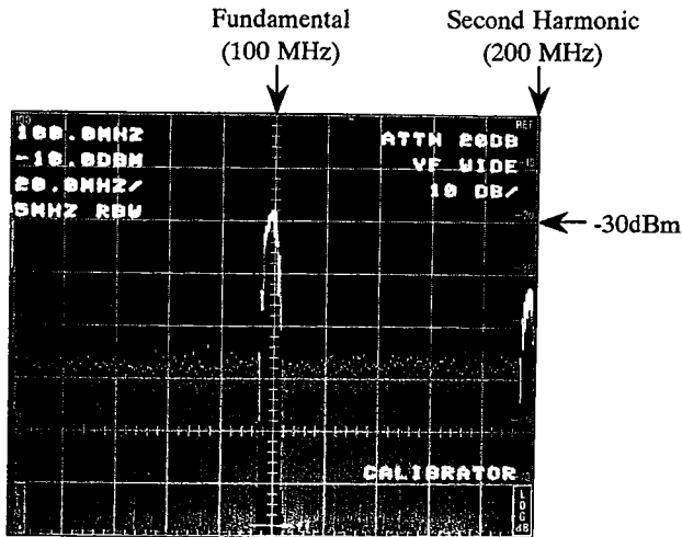
Figure 2-3. Calibration signal and second harmonic.
