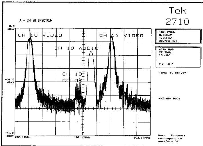
Figure 4-15. Typical plotter output from the 2710 showing a cable television spectrum.
