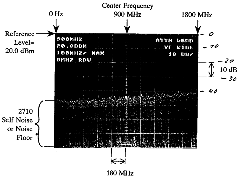
Figure 2-1. 2710 display with factory power-up settings.
