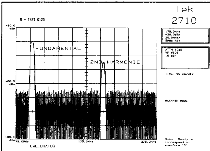
Figure 4-10. 2710 plot with title and plot labels.
