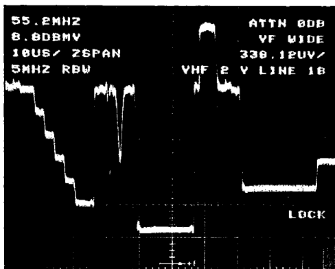
Figure 4-18. Video signal using knob-selectable horizontal line triggering (VITS visible).
