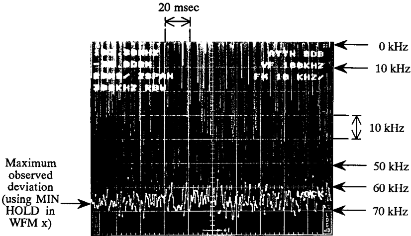
Figure 4-12. Instantaneous frequency deviation and maximum observed deviation.
