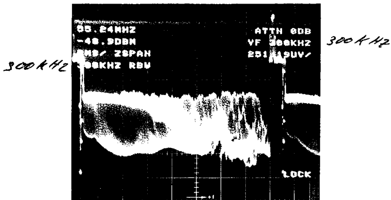
Figure 4-16. Video field using internal or TV field triggering.
