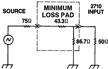
Figure 4-4. 75/50 ohm matching minimum loss pad.
