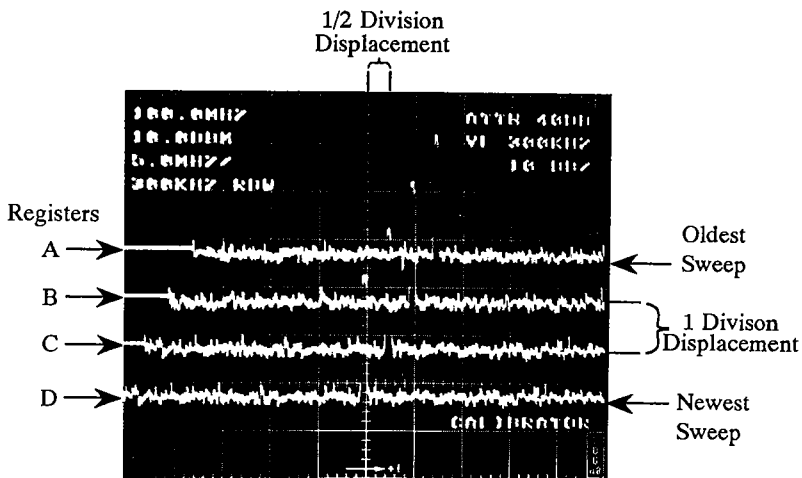
Figure 3-1. Example of a waterfall display.
